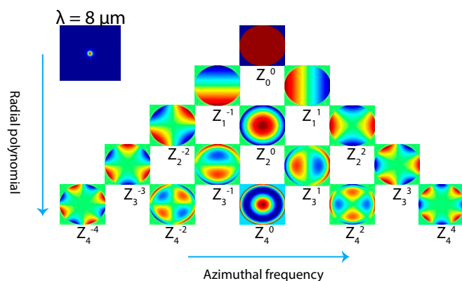
Fig. 2. Analysis of aberrations of the f = 19 mm lens ( NA = 0.371 ) at \lambda = 8 \mu\text{m} . The aberrations coefficients at other design wavelengths are included in SI Appendix .
